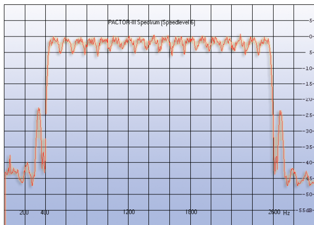
Spectrum of speedlevel 6 Bandwidth of the main spectrum: 2400 Hz @ -40 dB
